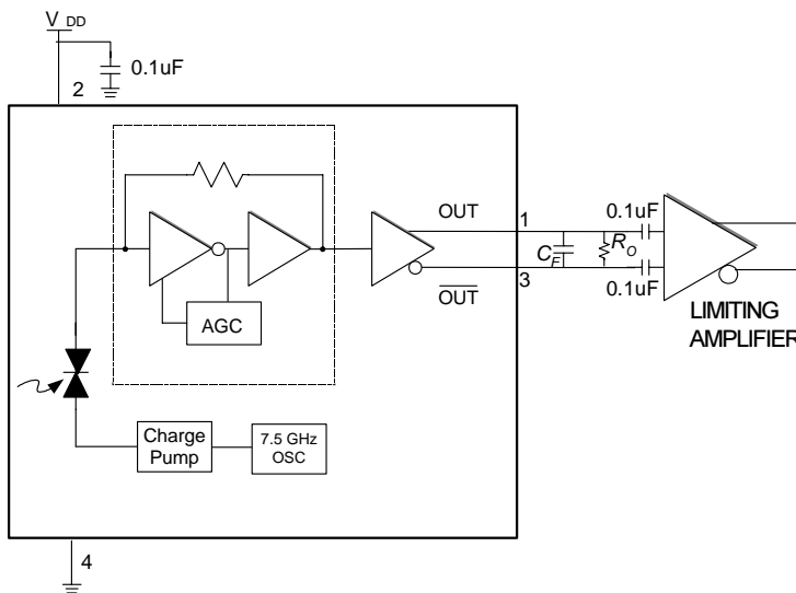
Figure 13: Application Schematic
